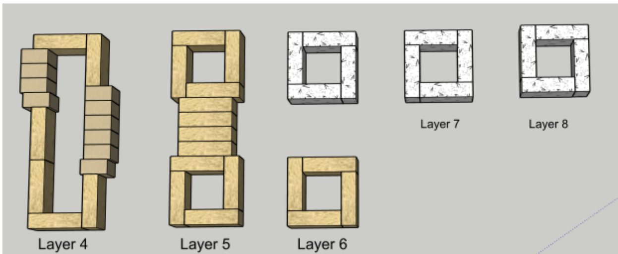
Brick Layers
